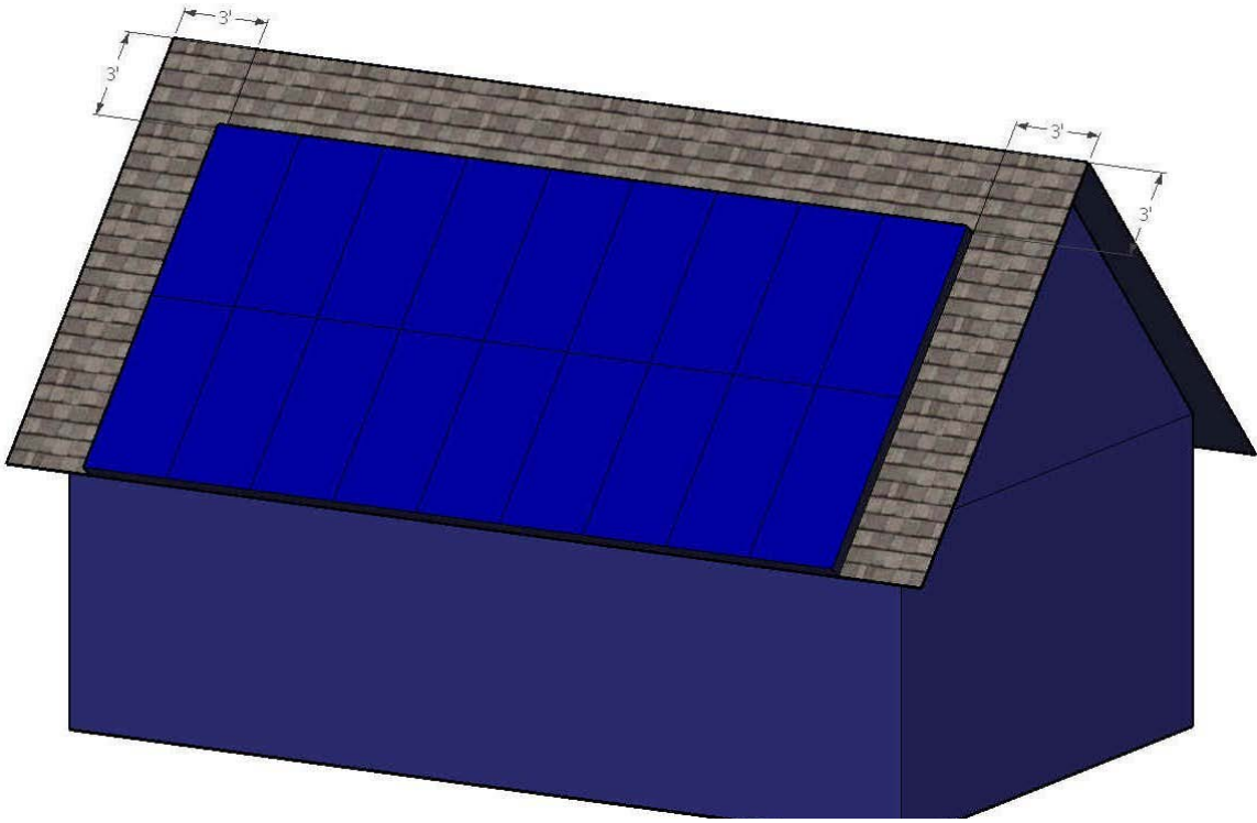
Diagram 3: Full Gable
